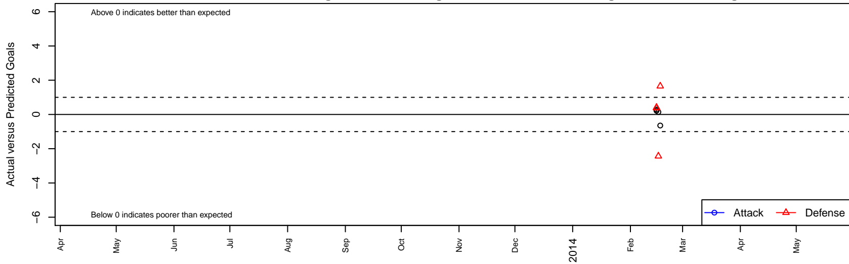
NM Rush 01 Nike B00 Dots are actual minus expected GF (blue circles) and GA (red triangles). Blue line is smoothed change in attack strength. Red is smoothed change in defense strength.
